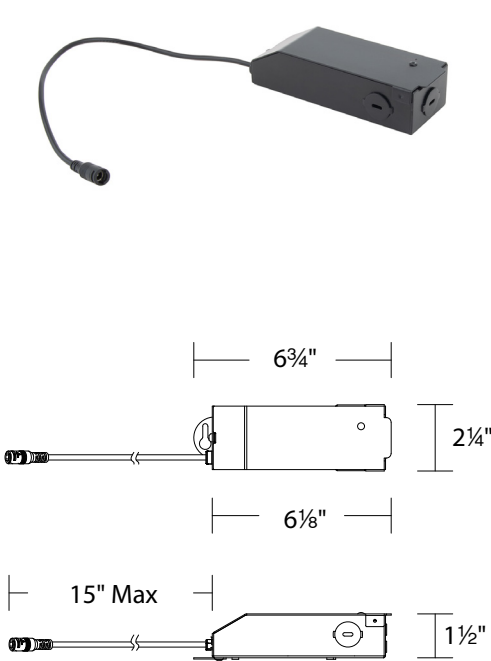
Applicable to 2 Cell Remodel Housing
