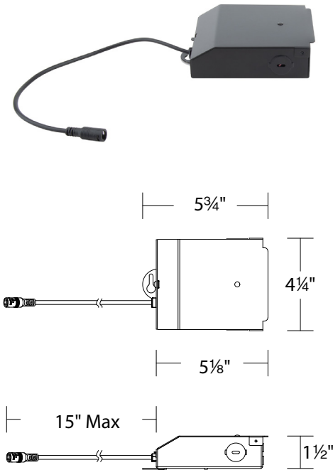
Applicable to 4 - 12 Cell Remodel Housings
