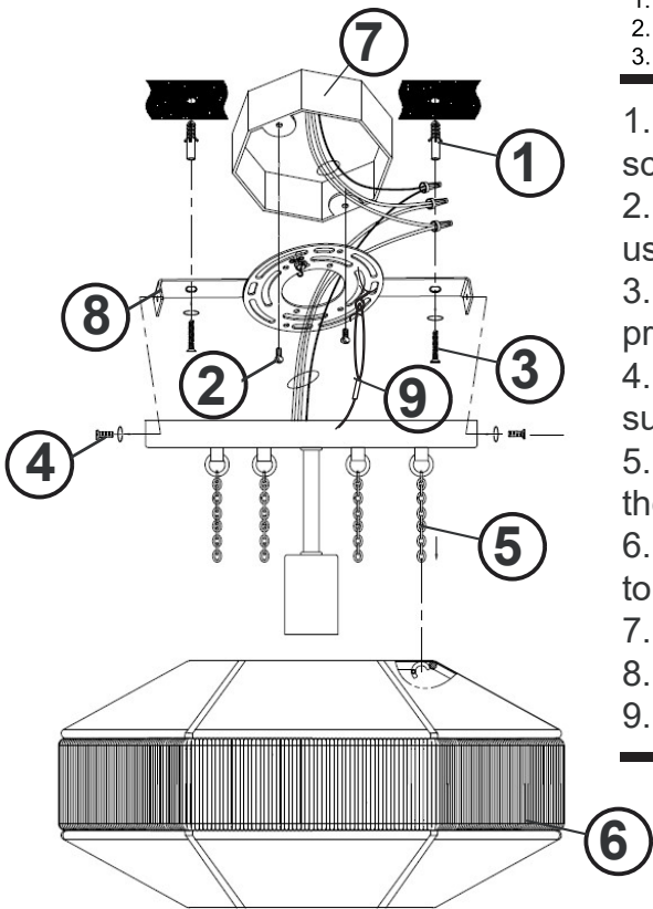
DRAWING 1- Mounting
