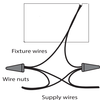
WIRING DIAGRAM
